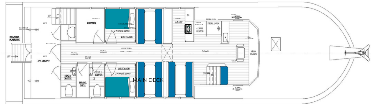
MAIN DECK
